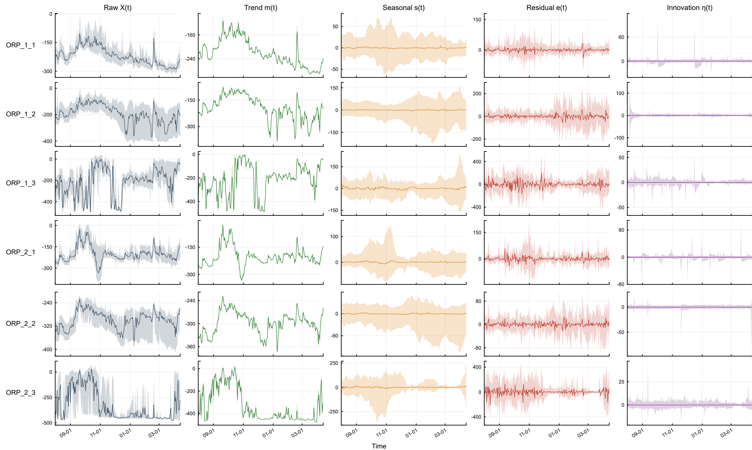
ORP channels (both trains) — full-span daily overview (min-max envelope) [2025-08-01~2026-04-13]
